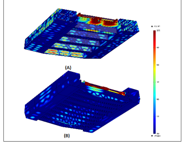
Figure 11. Vibration velocities ( L_v ) for an excitation of 1 N at a frequency of 141 Hz for the reference bridge (A) and the new bridge (B)
