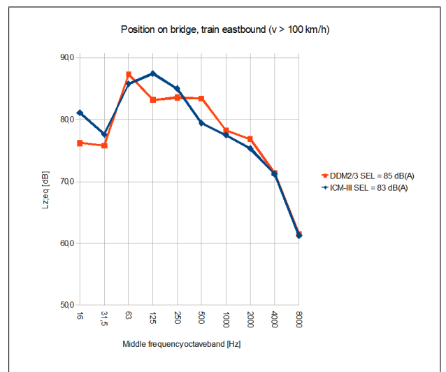
Figure 8. Spectral values of SEL at location 1 near the reference bridge for two types of trains
