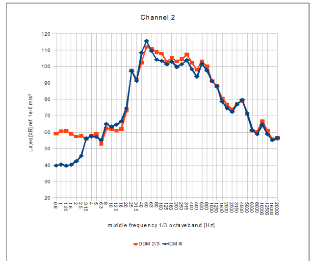
Figure 7. Spectral vibration acceleration at location 2 on the reference bridge for two types of trains.
