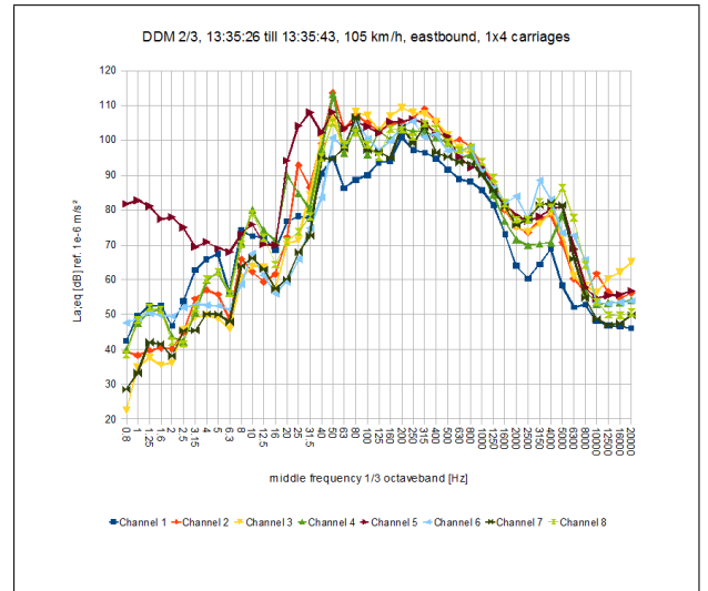
Figure 6. Spectral vibration acceleration of the passage of a train at eight locations on the reference bridge.
